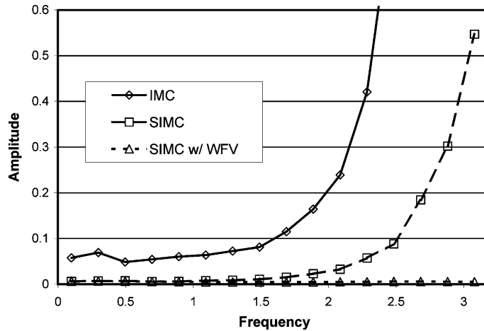
Fig. 6. Noise to signal ratio in the emission spectrum for fully biased collisionally pumped trap example.
