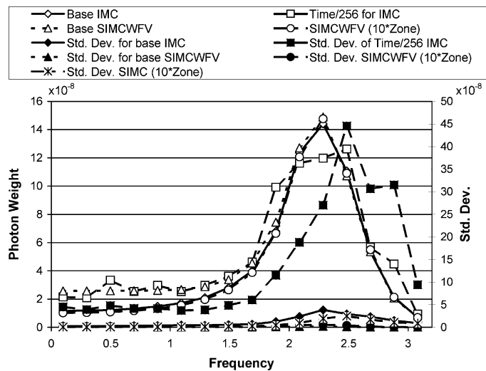
Fig. 8. Photon frequency distribution leaving the right side of the slab for surface heating example.
