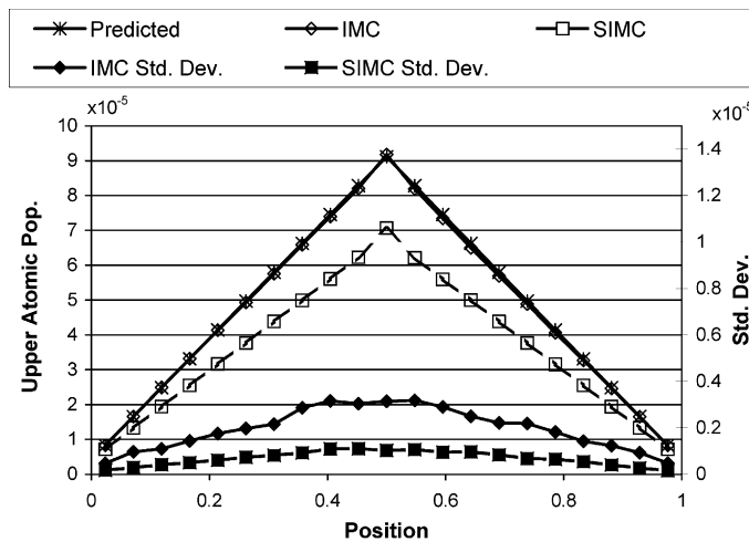
Fig. 12. Results for Milne’s problem.
