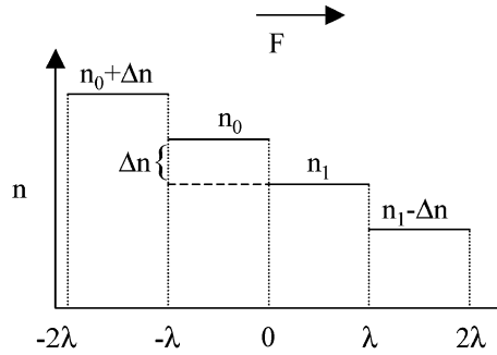
Fig. 13. Zoning diagram for Milne's problem.
