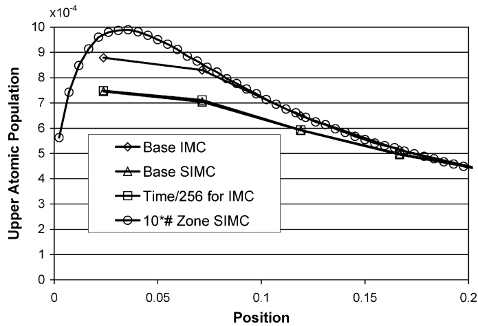
Fig. 7. Upper atomic population for the surface heating example at steady-state.
