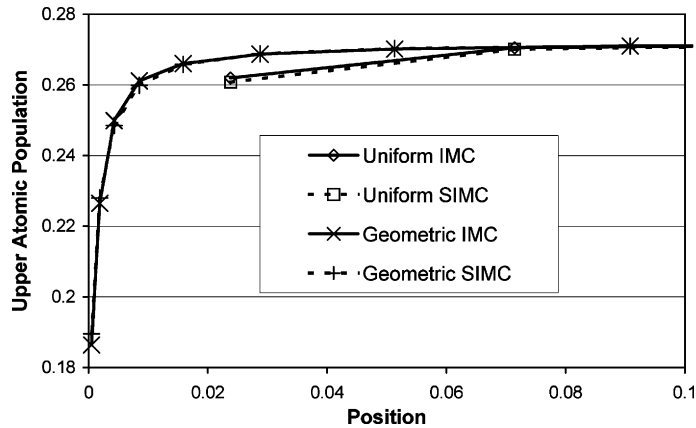
Fig. 2. Upper atomic population for collisionally pumped trap example.
