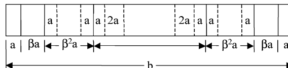
Fig. 1. Geometric zone and subzone construction.
