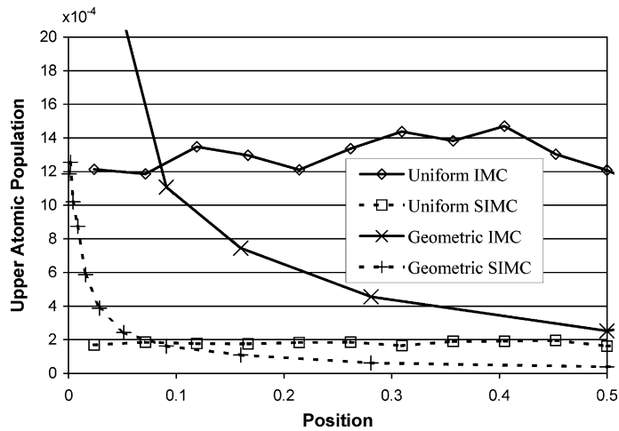
Fig. 3. Noise for upper atomic population for collisionally pumped trap example.
