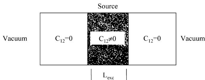
Fig. 11. Milne's problem layout.
